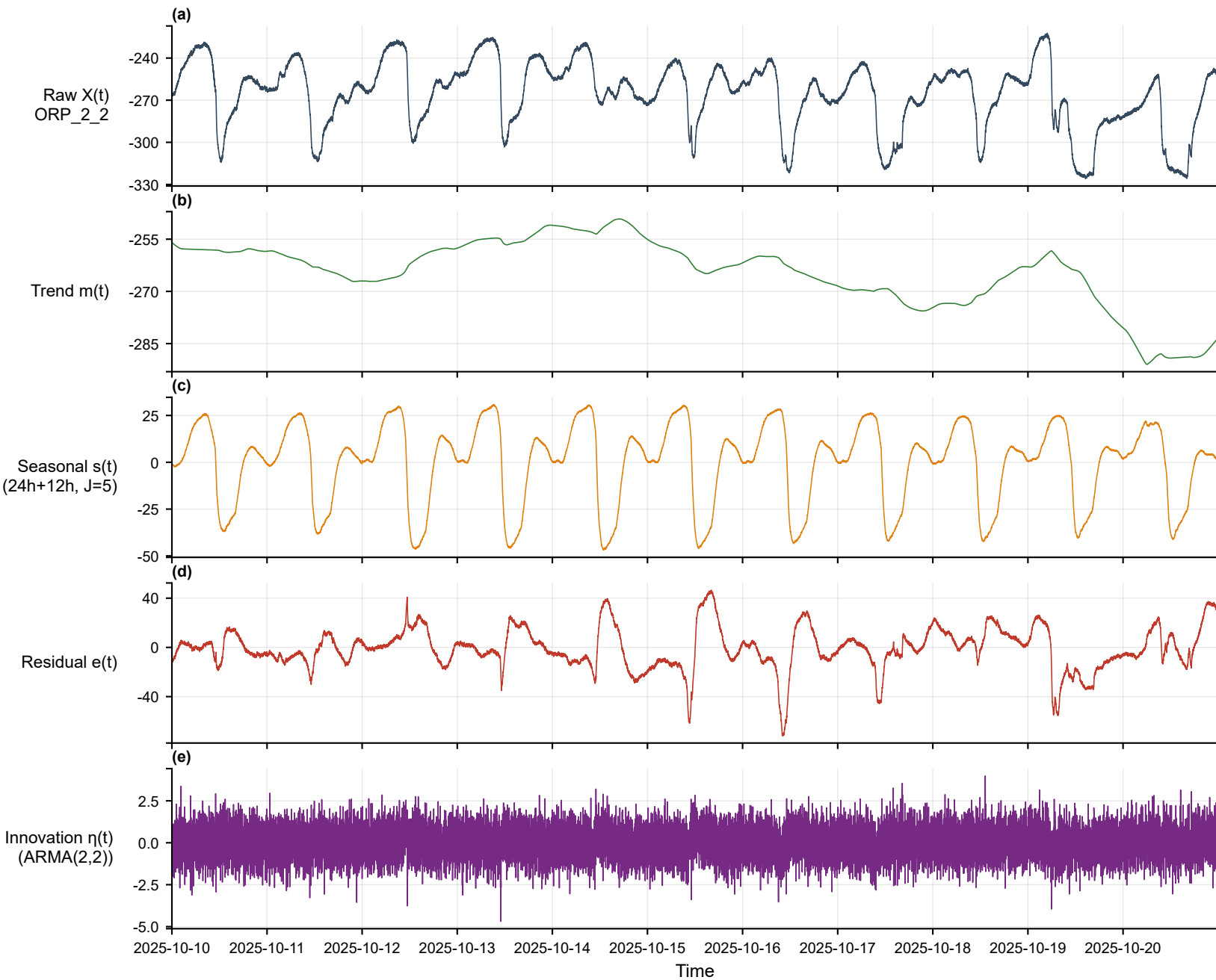
Multi-scale decomposition — ORP_2_2 (pre_anoxic_front, min) [2025-10-10~2025-10-20]
